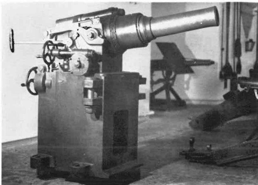
120 mm hurtigskydende stålhaubitx model 1893 i 120 mm kaponiereaffutage model 1893.
